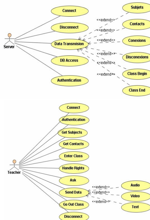
Figure 1: Use cases diagrams for the server module (on top) and for the teacher module of the application (at the bottom)
